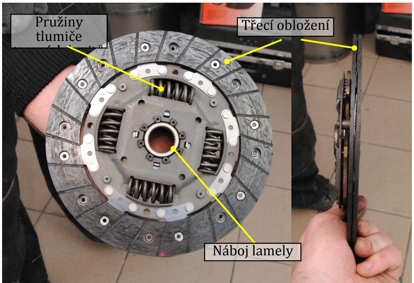
Obr. 7: Spojková lamela
